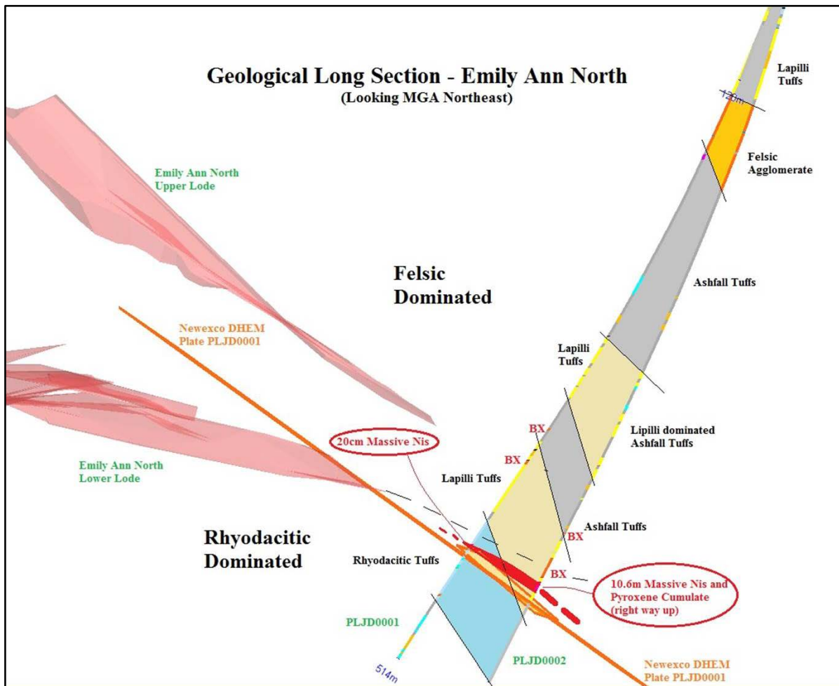
Figure 4: Geological section showing location of PLJD0001 & PLJD0002 nickel intersections relative to existing mineralisation. Mineralisation is open at depth and coincides with the structurally controlled plunge direction of Emily Ann mineralisation to the south
