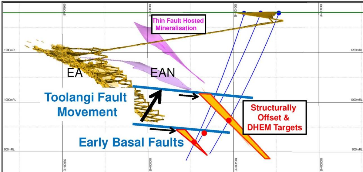
Figure 5: A cross section (looking north) shows the interpreted eastward horizontal offsets to the target zones which corresponds with modelled DHEM geophysical targets. Drilling (dark blue) is located ~800m north of the Emily Ann underground portal
